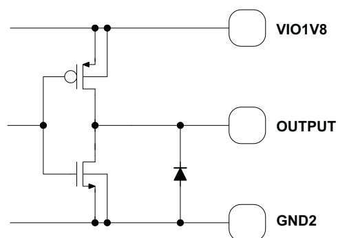
Figure 53. EXT_DC_DC_ON_OFF
