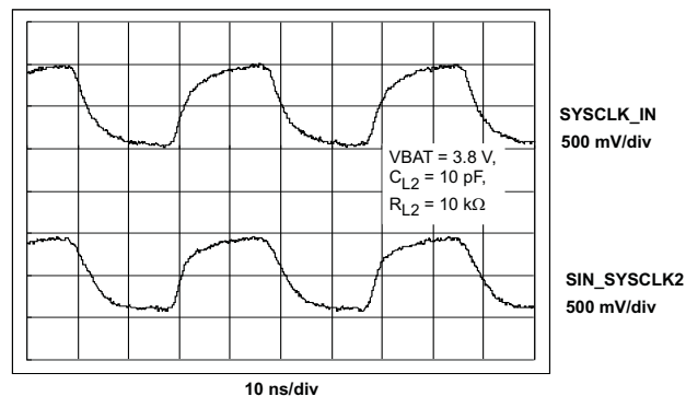
CLOCK DISTRIBUTION/SIN_SYSCLK2 INPUT vs OUTPUT (-1 dB TYP)
